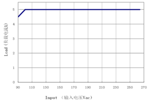
图 3-2-1 Load-Input derating curve (负载电流-输入电压降额曲线)
