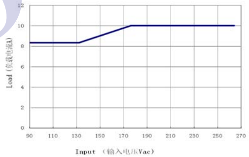
图3-2 Load-Input derating curve (负载电流—输入电压降额曲线)
