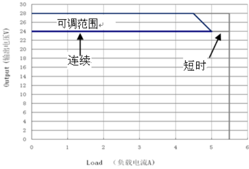
图 3-1-1 Output V-I curve (输出负载特性曲线)
